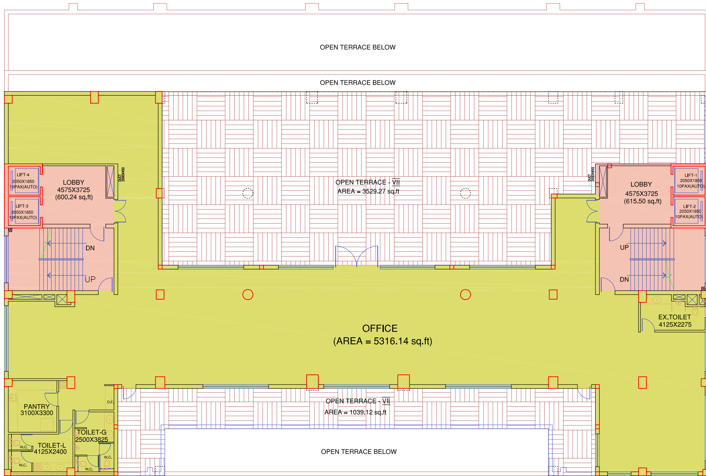
SEVENTH FLOOR PLAN TOTAL BUILT UP AREA (INCL. LIFT) = 6531.89 sq.ft
